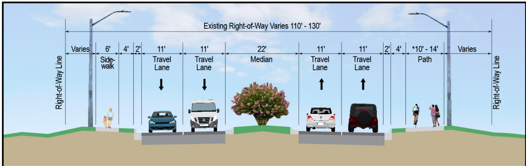
TYPICAL SECTION Chuluota Road Four-Lane Divided Section
